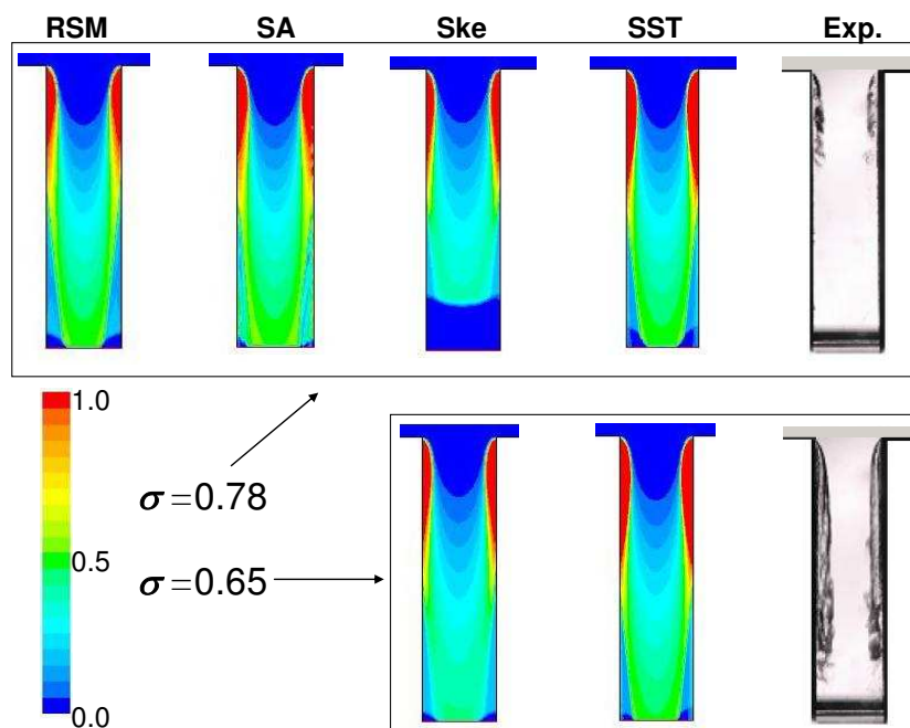
Fig 6: Comparison of CFD results obtained for the vapor fraction under two flow conditions, i.e., \sigma=0,78 and \sigma=0,65 , see Table 3, Sou et al., 2006 case. Notation: 0.0 – 1.0 values in the scale are for vapor fraction; \sigma = \sigma_{Sou} , see Eq. 2; RSM , Reynolds Stress Model; SA , Spalart Allmaras; Ske , Standard k-\epsilon ; SST , SST k-\omega .
