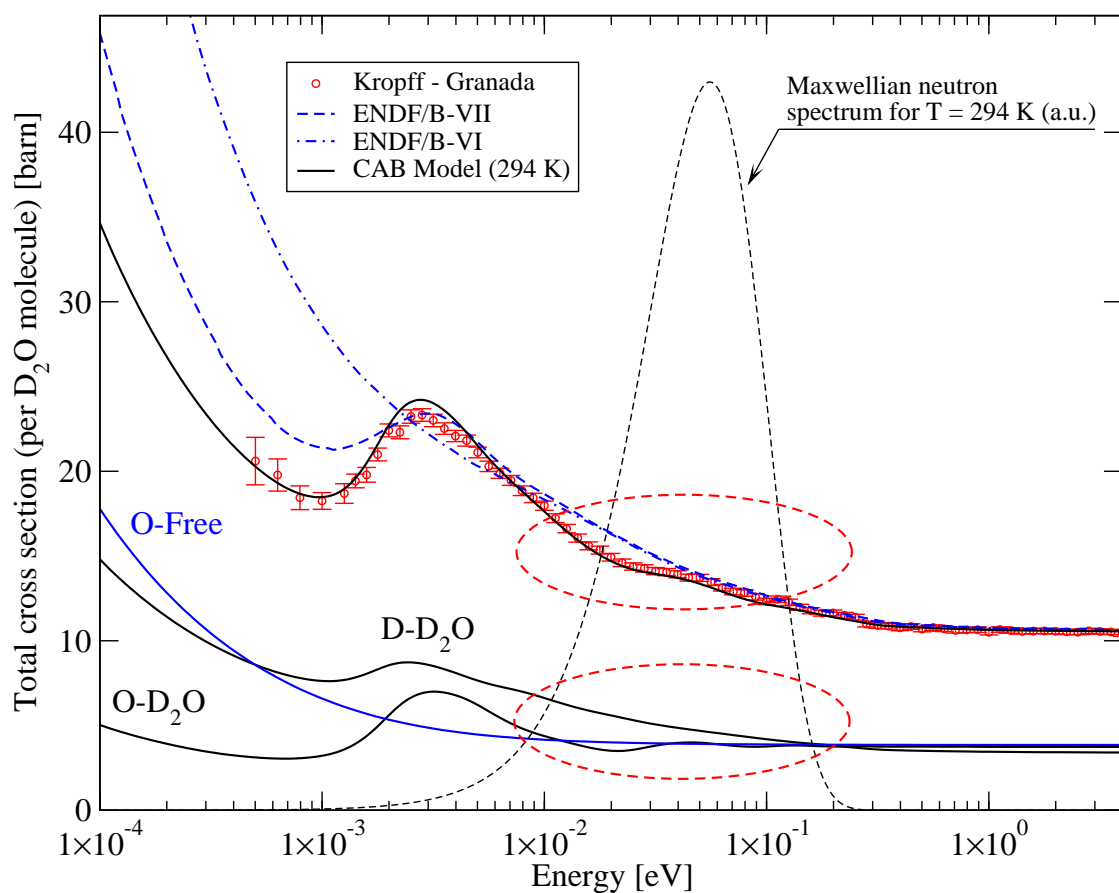
Figure 1: Total cross sections for heavy water at 294 K Kropff et al. (1974), compared with calculations using the CAB model, ENDF/B-VII (IKE model) and ENDF/B-VI (GA model) vs. the incident neutron energy. Ellipses mark the differences in the total cross sections at the energies which are very important for accurate modeling of the critical systems with the thermal neutron spectrum. The Maxwellian distribution for T_{\text{eff}} = 294 K, which would be expected for fully thermalized neutrons, is shown for reference. The differences in \sigma_{\text{tot}} can be traced to the total cross sections of O in \text{D}_2\text{O} (compare the curves at the bottom).
