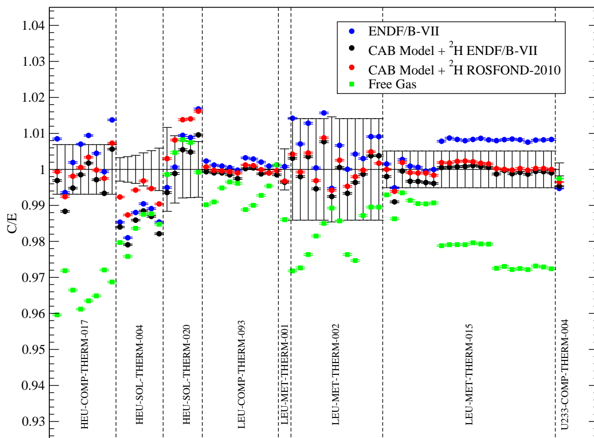
Figure 2: Calculation/Experiment ratio of the multiplication factor k_{\text{eff}} for 65 ICSBEP benchmarks modeling neutron criticality experiments in heavy water moderated systems.
