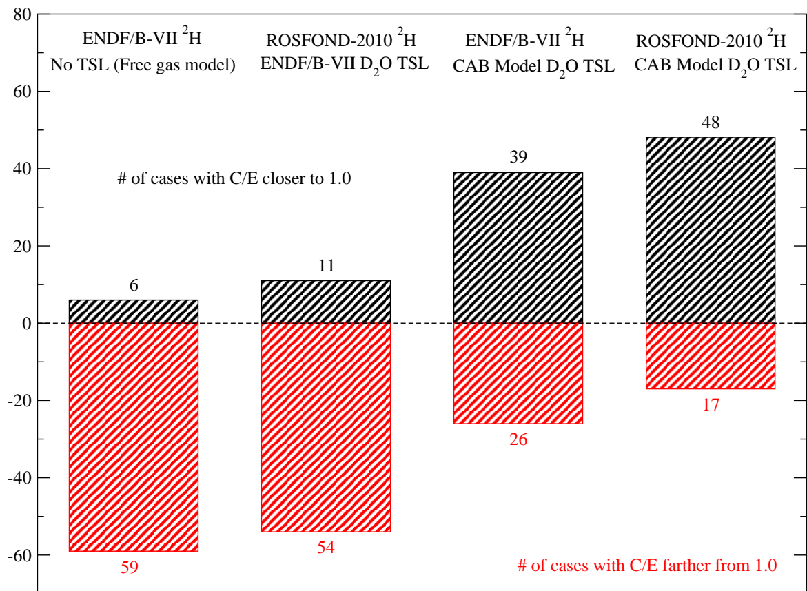
Figure 3: Comparison of different combinations of 2 H library and thermal scattering libraries for heavy water, against results with ENDF/B-VII.0 cross sections. Values above zero represent the number of benchmark cases that show an improvement in the result of C/E being closer to unity than calculations performed with the ENDF/B-VII.0-based library.
