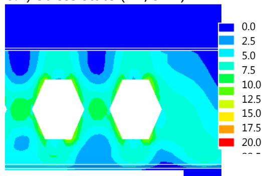
c.1) Stress state (kN/cm 2 )
