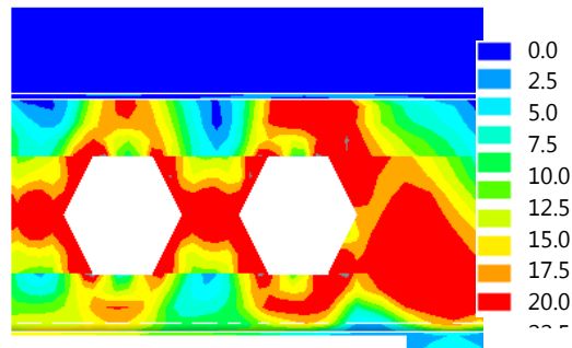
a.1) Stress state (kN/cm 2 )
