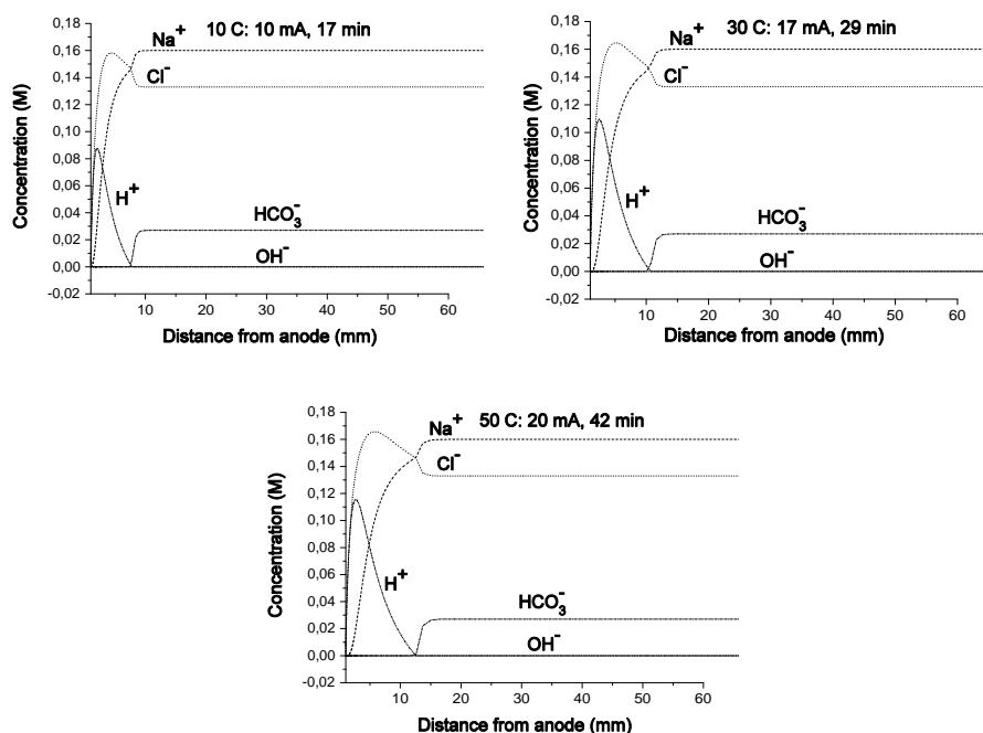
Figure 4: Buffered model simulations of sodium, chloride, hydrogen, hydroxile and bicarbonate ion concentration as a function of r after different dosages (10, 30 and 50 C) of EChT.
