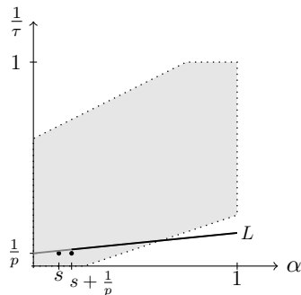
FIGURE 2. The black segment in the line L shows the improved regularity with data associated to (s, \frac{1}{p}) \in \mathcal{R}_\varepsilon when d = 10 .
